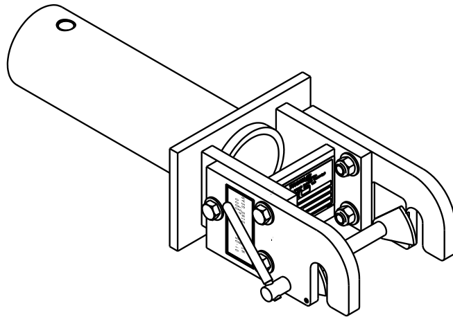
Model: 01-0535-0000 Towbar Head Attachment Bell 214ST (with landing gear)
