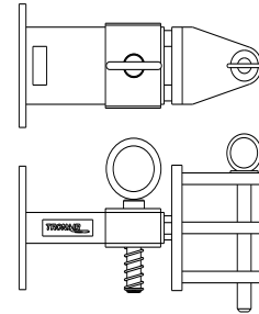
FIGURE 3 01-1950-5000 Standard Telecoupler
