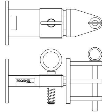
FIGURE 3 01-1950-5000 Standard Telecoupler
