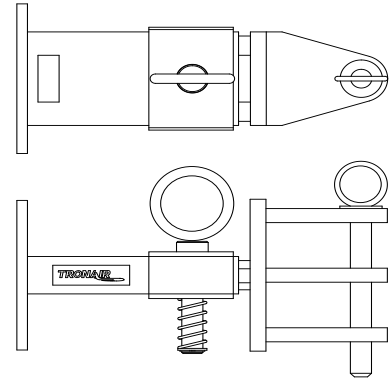
FIGURE 3 01-1950-5000 Standard Telecoupler
