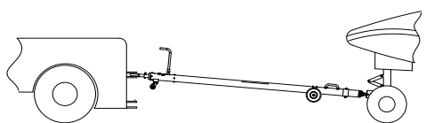
Incorrect Excessive Towbar Angle
