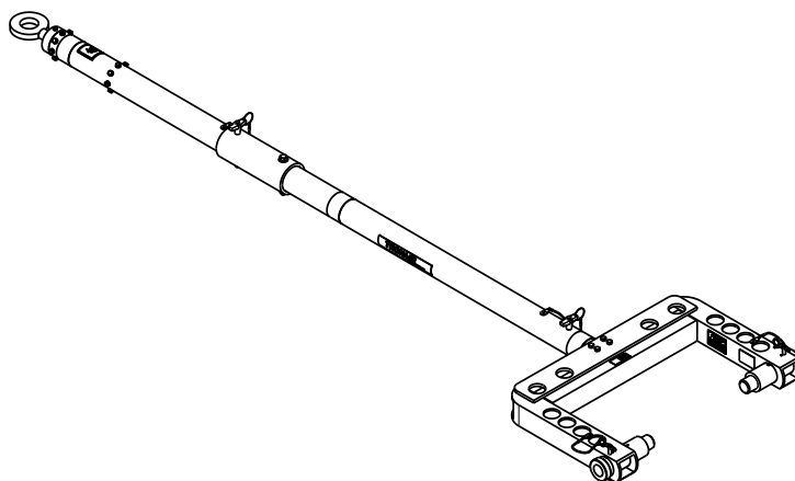
Model: 01-1261-0011 Portable Towbar Gulfstream GII, GIII, GIV, GV
