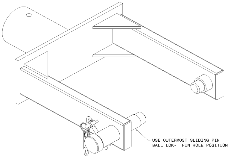
FIGURE 6 – Sliding Pin Position for Cessna Citation
