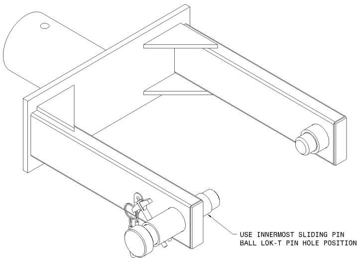
FIGURE 7 – Sliding Pin Position for Learjet
