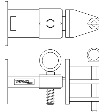
FIGURE 4 01-1950-5000 Standard Telecoupler
