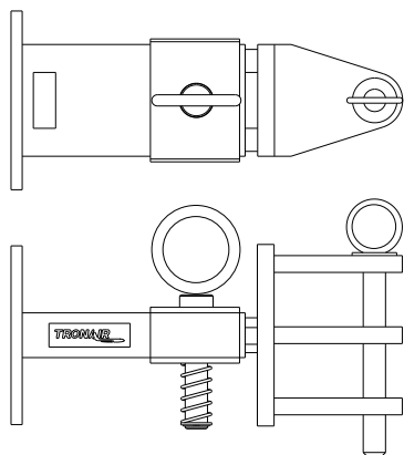
FIGURE 3 01-1950-5000 Standard Telecoupler
