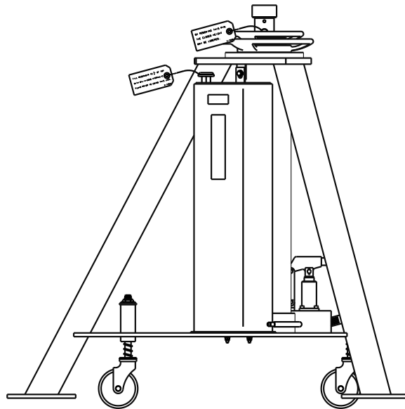
Model: 02-7842C0100 12 Ton Two Stage Jack
