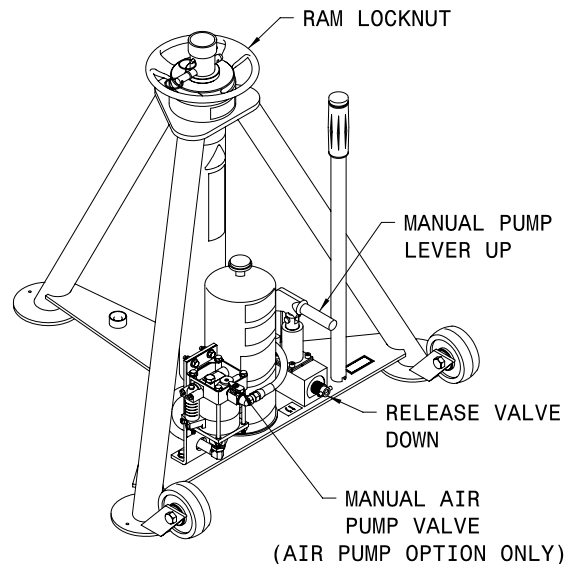
FIGURE 7.3 – Operator Controls
