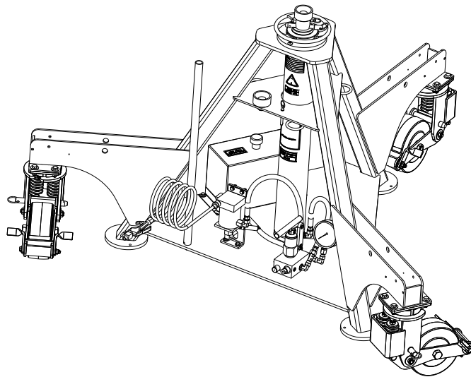
Model: 02A7914C0110 10 Ton Single Stage Jack
