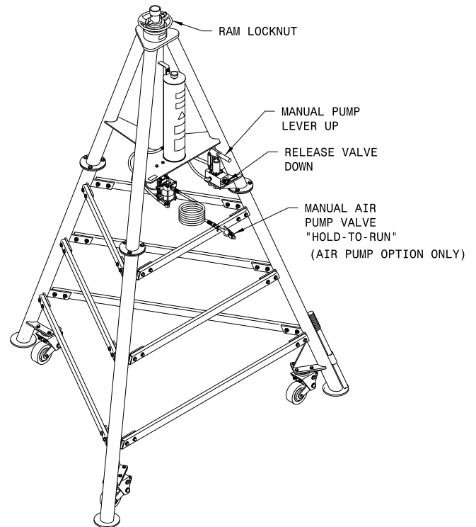
FIGURE 3 – Operator Controls Locations
