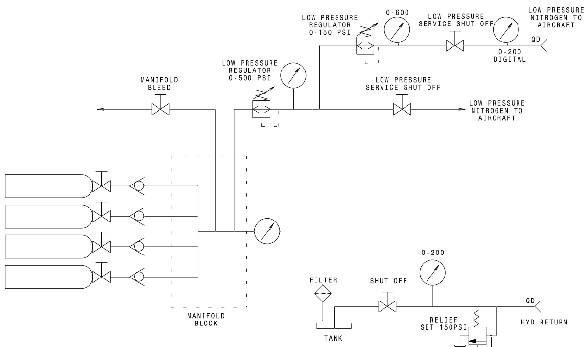
Figure 1 - Schematic
