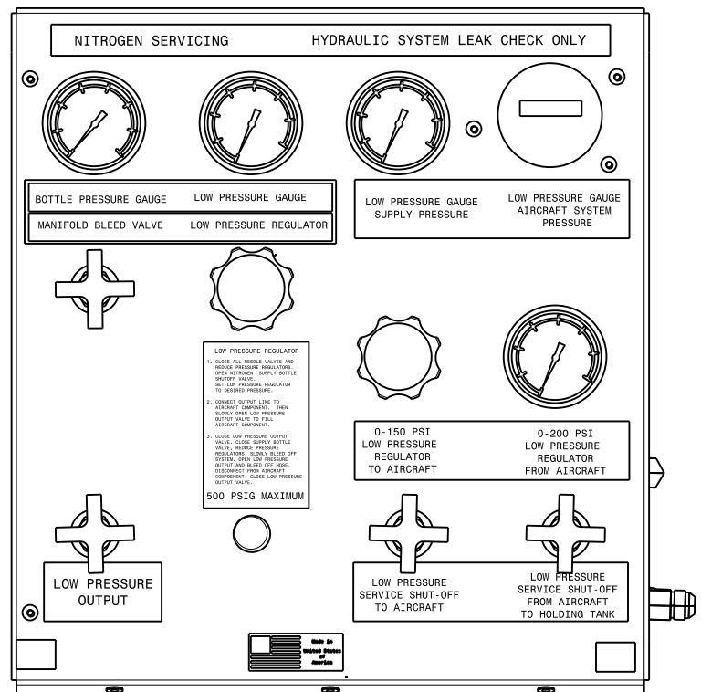
FIGURE 8 - Instrument Panel
