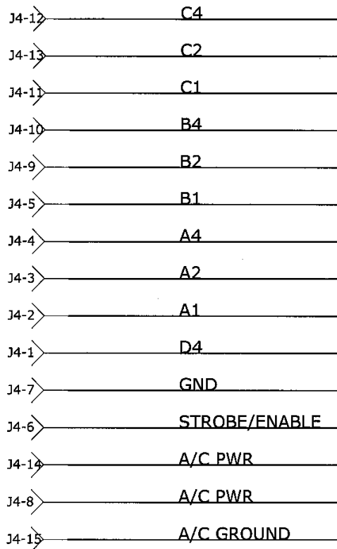
Figure 3-4 J4 Pinout
