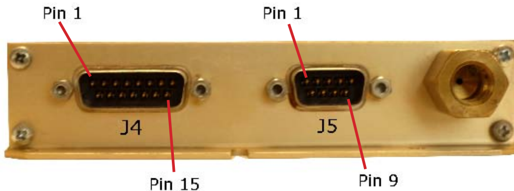
Figure 3-2 J4/J5 Connector Pins
