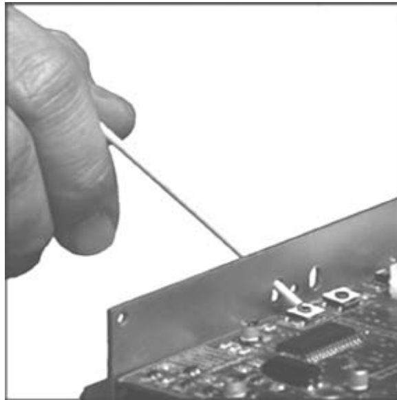
Figure 3-8 SAE 5-35 Adjustment
