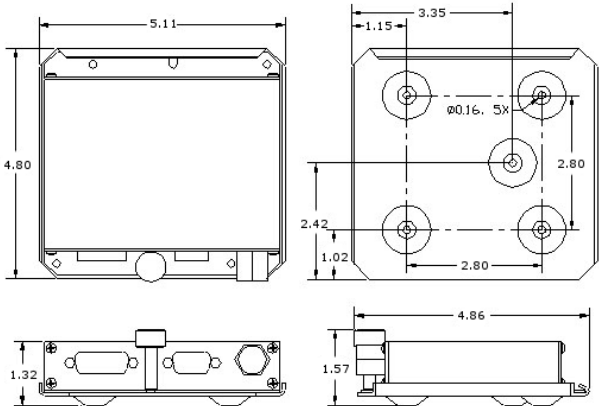
Figure 3-1 SAE5-35 Outline Dimensions (with tray)
