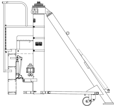
Model: 8760 Two Stage Fixed Height Hydro – Mechanical Aviation Tripod jack
