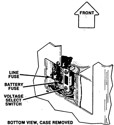
BOTTOM VIEW, CASE REMOVED
