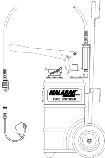
Model: PF53481-140P 5 gal (18.9 l) Fluid Dispenser
