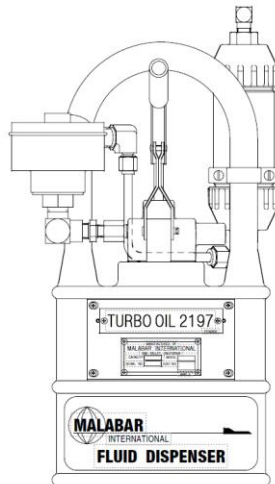
Model: PF55966-6PWS 2 gal (7.6 l) Fluid Dispenser
